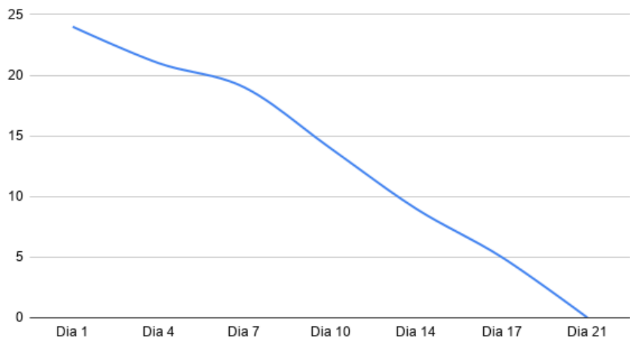
Burn-down Chart
